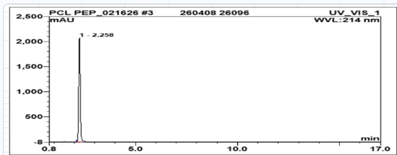
HPLC Chromatogram (Retention Time: 2.258 min)
